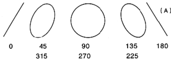
Fig.5 Measurement of Phase Characteristic
